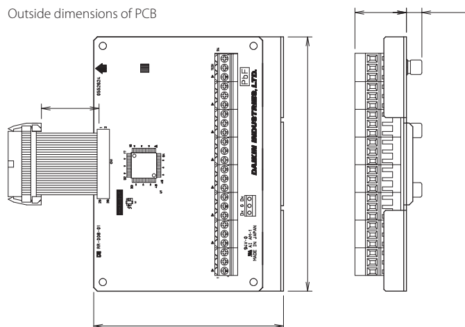
Outside dimensions of PCB
