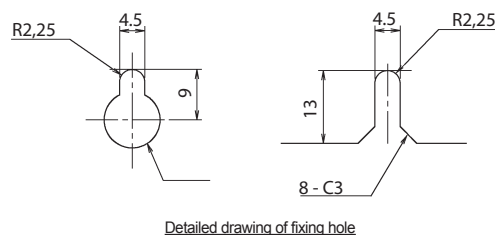
Detailed drawing of fixing hole
