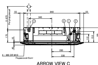
ARROW VIEW C
