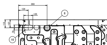
View C
